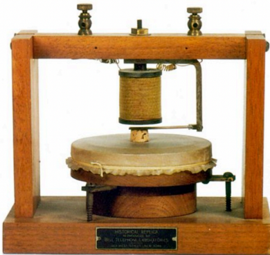
Alexander's first telephone that worked (1875). However, the sound wasn't clear enough.
